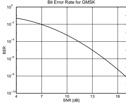
Figure 10. The bit error rate vs. signal to noise ratio
